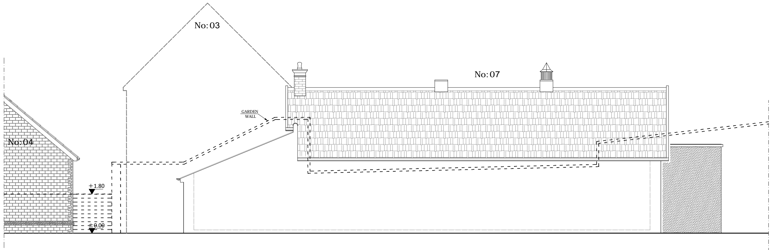
EXISTING REAR ELEVATION SCALE: 1/100
